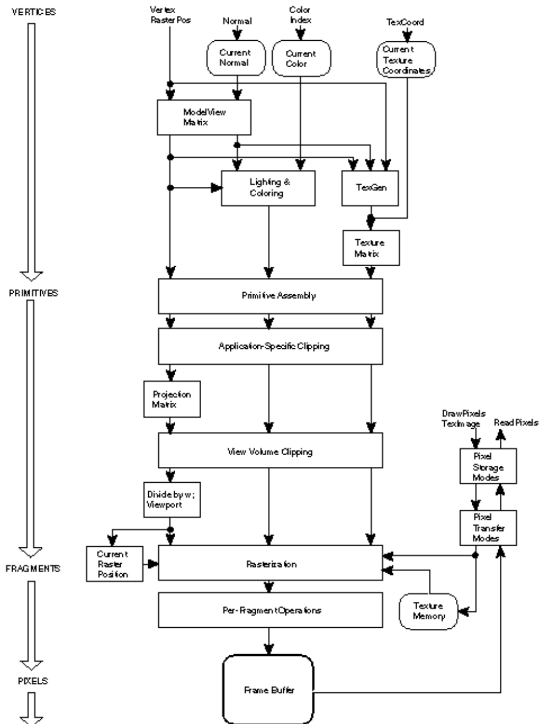
Figure 2–1 OpenGL Pipeline
