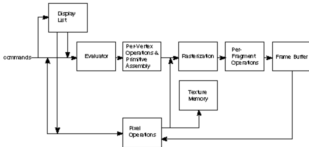
Figure 1–1 OpenGL Block Diagram
